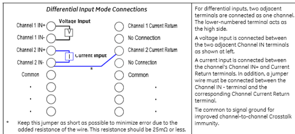
Figure 3: Field Wiring - Differential Mode
